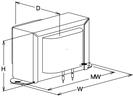
Horizontal Mount
