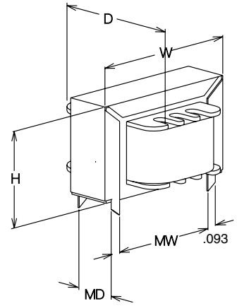
Horizontal Mount with P.C. Board Tabs
