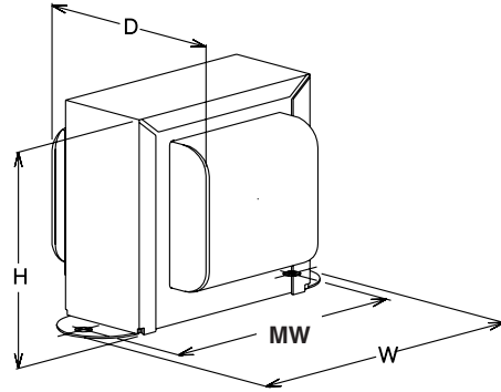
Vertical Mount
