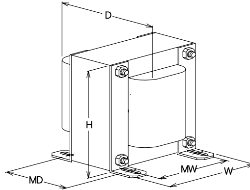
Horizontal Foot Mount
