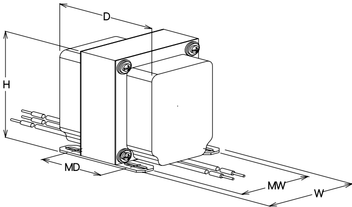
Foot Mounted Metal End Bells
